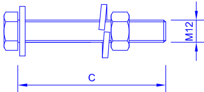
14 15 16 M12xC+P(1)+AP(1)+AM(1) (Esc. 1/2)
