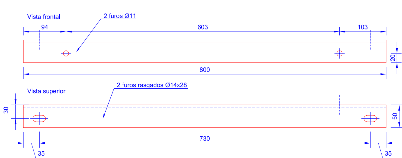
1d L50x50x5 (Esc. 1/5)
