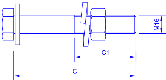
11 12 13 M16xCxC1+P(1)+AP(1)+AM(1) (Esc. 1/2)
